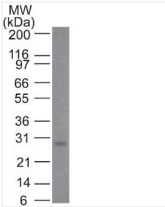
WB (Western Blot) Western Blot of Bcl-2 in human Skin using Bcl-2 Monoclonal Antibody (SPM530).
