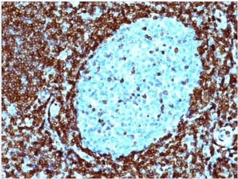
IHC (Immunohistochemistry) Formalin-fixed, paraffin-embedded human non-Hodgkin's Lymphoma stained with Bcl-2 Monoclonal Antibody (SPM530).
