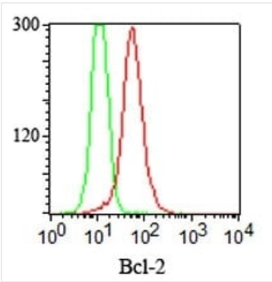
FCM/FACS (Flow Cytometry) Flow Cytometry of Jurkat cells using Bcl-2 Monoclonal Antibody (SPM530) (red) and isotype control (green).
