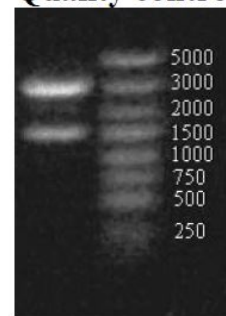
RES:HindIII
