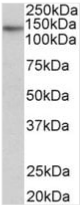
WB (Western Blot) 0.5ug/ml) staining of Human Skeletal Muscle lysate (35ug protein in RIPA buffer). Primary incubation was 1 hour. Detected by chemiluminescence.
