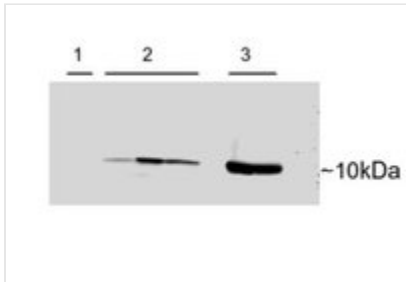
WB (Western Blot) 0.15ug/ml) staining of adenovirus-mediated gene transfer in rat heart cells 1) Untransfected, 2) transient transfection with Human PVALB.3) Untransfected rat skeletal muscle. Primary incubation was 1 hour. Detected by chemiluminescence.
