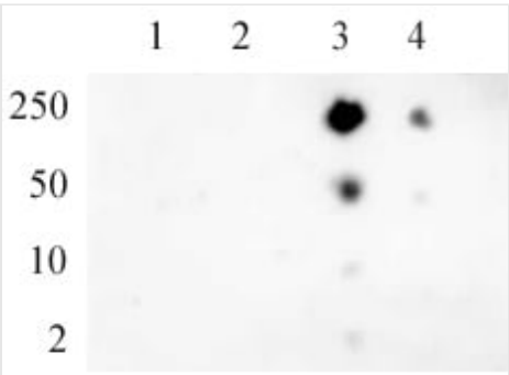
DB (Dot Blot) RNA pol II CTD phospho Ser5 pAb tested by dot blot analysis. Dot blot analysis was used to confirm the specificity of RNA pol II CTD phospho Ser5 antibody for phospho-Ser5 of the RNA Pol II C-terminal domain heptad repeat. Modified and unmodified peptides were spotted onto PVDF and probed with the antibody at a dilution of 0.2 ug/ml. Decreasing amounts of peptide were spotted in each row. Lane 1: Peptide phosphorylated at CTD repeat serine 2. Lane 2: Unmodified CTD repeat serine 2 peptide. Lane 3: Peptide phosphorylated at CTD repeat serine 5. Lane 4: Unmodified CTD repeat serine 5 peptide.
