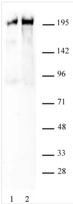
WB (Western Blot) RNA pol II CTD phospho Ser5 antibody tested by Western blot. Nuclear extract of HeLa cells (20 ug) probed with RNA pol II CTD phospho Ser5 antibody at a dilution of 0.5 ug/ml.
