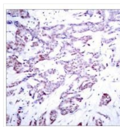
IHC (Immunohistochemistry)
