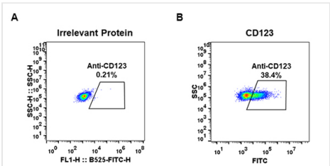
FCM/FACS (Flow Cytometry) Figure 1. Expi 293 cell line transfected with irrelevant protein (left) and human CD123(right) were surface stained with Rabbit anti-CD123 monoclonal antibody 1ug/ml ( clone: DM33) followed by Alexa 488-conjugated anti-rabbit IgG secondary antibody.
