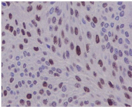
IHC (Immunohiostchemistry) Immunohistochemical analysis of paraffin-embedded human bladder, using Cyclin D1 Antibody(AAA46888)CCND1 was detected in paraffin-embedded tissue section. Heat mediated antigen retrieval was performed in citrate buffer (pH6, epitope retrieval solution) for 20 mins. The tissue section was blocked with 10% goat serum. The tissue section was then incubated with 1ug/ml rabbit anti-CCND1 Antibody (AAA46888)overnight at 4 degree C. Biotinylated goat anti-rabbit IgG was used as secondary antibody and incubated for 30 minutes at 37 degree C. The tissue section was developed using Streptavidin-Biotin-Complex (SABC) with DAB as the chromogen.
