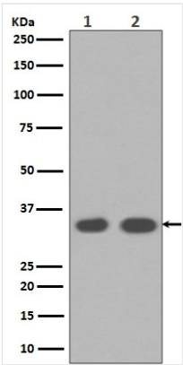
WB (Western Blot) Western blot analysis of Cyclin D1 expression in (1)MCF-7 cell lysates;(2) LnCaP cell lysates (AAA46888).Electrophoresis was performed on a 5-20% SDS-PAGE gel at 70V (Stacking gel) / 90V (Resolving gel) for 2-3 hours. The sample well of each lane was loaded with 50ug of sample under reducing conditions.After Electrophoresis, proteins were transferred to a Nitrocellulose membrane at 150mA for 50-90 minutes. Blocked the membrane with 5% Non-fat Milk/ TBS for 1.5 hour at RT. The membrane was incubated with rabbit anti-CCND1 monoclonal antibody overnight at 4 degree C, then washed with TBS-0.1%Tween 3 times with 5 minutes each and probed with a goat anti-rabbit IgG-HRP secondary antibody at a dilution of 1:10000 for 1.5 hour at RT. The signal is developed using an Enhanced Chemiluminescent detection (ECL) kit with Tanon 5200 system. A specific band was detected for CCND1
