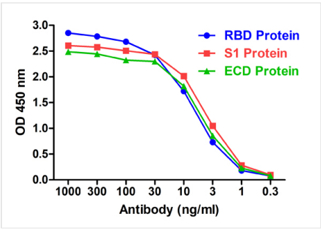
ELISA Figure 2 ELISA Validation with SARS-CoV-2 (COVID-19) Spike RBD, S1 and ECD Proteins Antibodies: SARS-CoV-2 (COVID-19) Spike S1 RBD Antibody, AAA40983. A direct ELISA was performed using SARS-CoV-2 Spike recombinant proteins (RBD, 10-303; S1, 97-087; ECD, 11-070) as coating antigen at 1ug/mL and the anti-SARS-CoV-2 (COVID-19) Spike S1 RBD antibody (AAA40983) as the capture antibody, following by anti-cMyc-tag antibody (PM-7669) at 1ug/mL. Secondary: Goat anti-mouse IgG HRP conjugate at 1:5000 dilution. Detection range is from 0.3 ng/mL to 1000 ng/mL. SARS-CoV-2 (COVID-19) Spike S1 RBD Antibody, AAA40983 can detect spike RBD, S1 and ECD proteins at 2 ng/mL.
