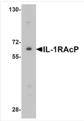
WB (Western Blot) Western blot analysis of IL-1RAcP expression in K562 cell lysate with IL-1RAcP antibody at 1 &#956;g/mL.
