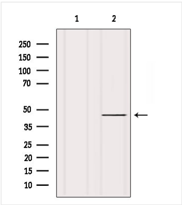
WB (Western Blot) Western blot analysis of extracts from Mouse brain, using p38 MAPK Antibody. Lane 1 was treated with the blocking peptide.
