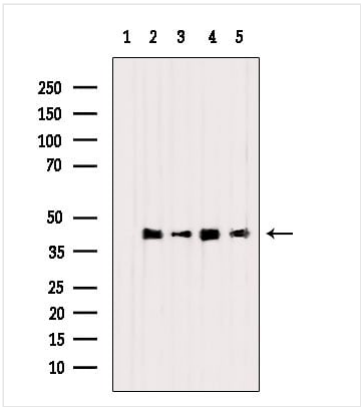
WB (Western Blot) Western blot analysis of extracts from various samples, using p38 MAPK Antibody. Lane 1: Mouse brain lysates treated with blocking peptide; Lane 2: Mouse brain lysates; Lane 3: Hybridoma cell lysates; Lane 4: Hela cell lysates; Lane 5: Vero cell lysates.
