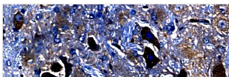
IHC (Immunohistochemistry)
