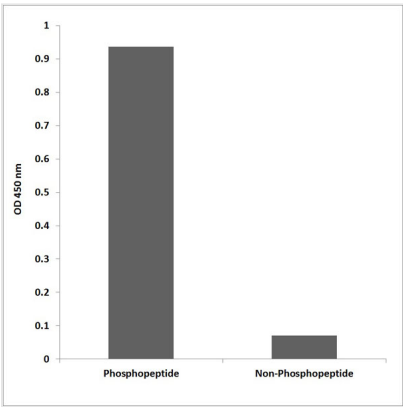
ELISA Enzyme-Linked Immunosorbent Assay (Phospho-ELISA) for Immunogen Phosphopeptide (Phospho-left) and Non-Phosphopeptide (Phospho-right), using Mnk1 (Phospho-Thr385) Antibody
