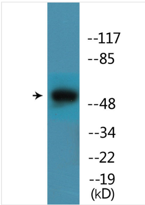
WB (Western Blot) Western blot analysis of lysates from COLO205 cells treated with PMA 125ng/ml 30', using Mnk1 (Phospho-Thr385) Antibody.
