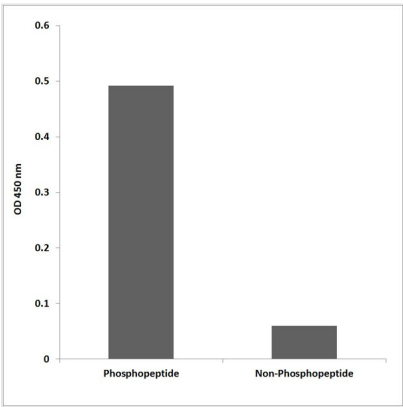
ELISA Enzyme-Linked Immunosorbent Assay (Phospho-ELISA) for Immunogen Phosphopeptide (Phospho-left) and Non-Phosphopeptide (Phospho-right), using HER2 (Phospho-Tyr1112) Antibody
