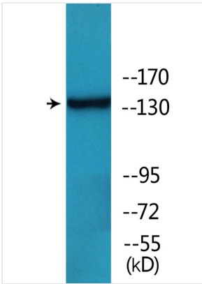
WB (Western Blot) Western blot analysis of lysates from HepG2 cells treated with PMA 125ng/ml 20', using HER2 (Phospho-Tyr1112) Antibody.
