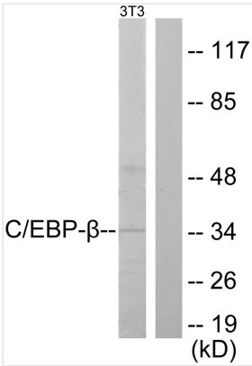
WB (Western Blot) Western blot analysis of lysates from NIH/3T3 cells, using C/EBP-beta Antibody. The lane on the right is blocked with the synthesized peptide.
