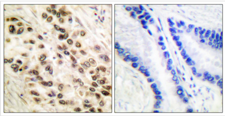
IHC (Immunohistochemistry) Immunohistochemistry analysis of paraffin-embedded human lung carcinoma tissue, using C/EBP-beta Antibody. The picture on the right is blocked with the synthesized peptide.
