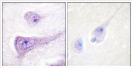
IHC (Immunohistochemistry) Immunohistochemistry analysis of paraffin-embedded human brain, using WASP (Phospho-Tyr290) Antibody. The picture on the right is blocked with the phospho peptide.
