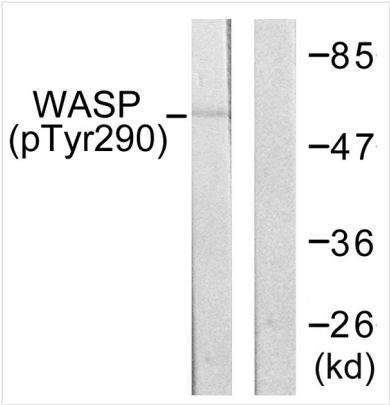
WB (Western Blot) Western blot analysis of lysates from HepG2 cells, using WASP (Phospho-Tyr290) Antibody. The lane on the right is blocked with the phospho peptide.
