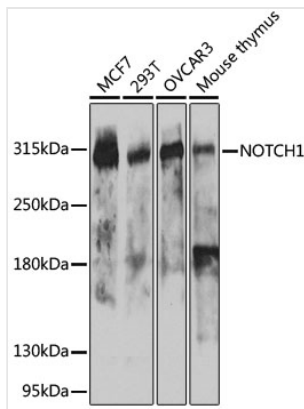
WB (Western Blot) Western blot analysis of extracts of various cell lines, using NOTCH1 antibody.
