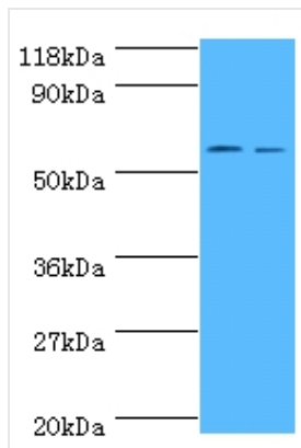
WB (Western Blot) All lanes: Carboxylesterase 1C antibody at 2ug/ml
