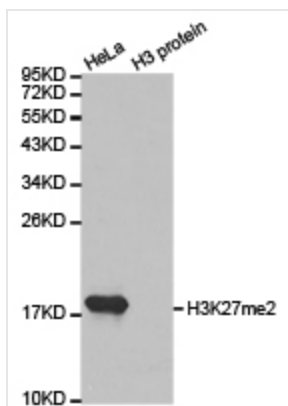
WB (Western Blot) Western blot analysis of extracts of HeLa cell line and H3 protein expressed in E. coli., using H3K27me2antibody.
