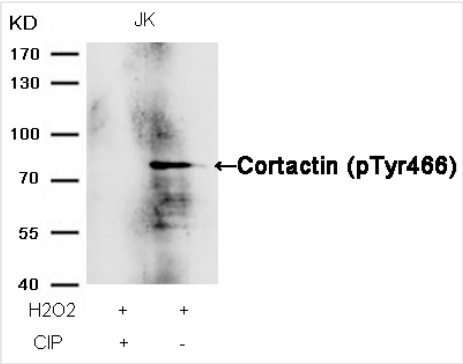
WB (Western Blot) Western blot analysis of extracts from JK cells, treated with H2O2 or calf intestinal phosphatase (CIP), using Cortactin (Phospho-Tyr466) Antibody.
