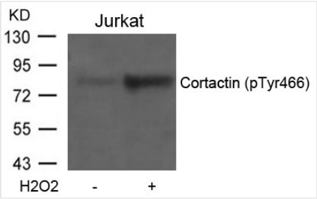
WB (Western Blot) Western blot analysis of extracts from Jurkat cells untreated or treated with H2O2 using Cortactin(Phospho-Tyr466) Antibody.
