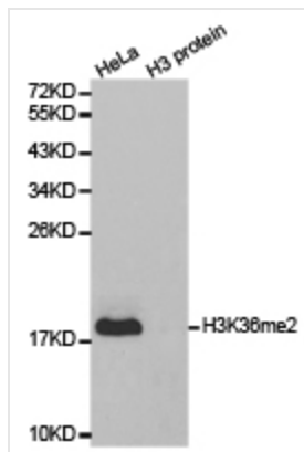
WB (Western Blot) Western blot analysis of extracts of HeLa cell line and H3 protein expressed in E. coli., using H3K36me2 antibody.
