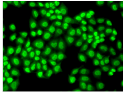
IF (Immunofluorescence) Immunofluorescence analysis of HeLa cell using GTF2F1 antibody.
