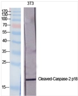
WB (Western Blot) Western Blot analysis of NIH-3T3 cells using Cleaved-Caspase-2 p18 (G170) Polyclonal Antibody
