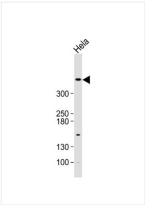
WB (Western Blot) Anti-ATM Antibody (C12) at 1:500 dilution + HeLa whole cell lysateLysates/proteins at 20 ug per lane.SecondaryGoat Anti-Rabbit IgG, (H+L), Peroxidase conjugated at 1/10000 dilution.Predicted band size : 351 kDaBlocking/Dilution buffer: 5% NFD/MTBST.
