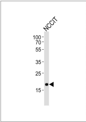
WB (Western Blot) Western blot analysis of lysate from NCCIT cell line, using Mouse Hmga2 Antibody (N-term). AAA290302 was diluted at 1:1000. A goat anti-rabbit IgG H&L(HRP) at 1:10000 dilution was used as the secondary antibody. Lysate at 20ug.
