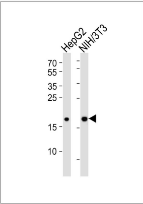
WB (Western Blot) Western blot analysis of lysates from HepG2, mouse NIH/3T3 cell line (from left to right), using Mouse Hmga2 Antibody (N-term). AAA290302 was diluted at 1:1000 at each lane. A goat anti-rabbit IgG H&L(HRP) at 1:10000 dilution was used as the secondary antibody. Lysates at 20ug per lane.
