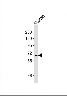
WB (Western Blot) Anti-MeCP2 Antibody (S421) at 1:1000 dilution + mouse brain lysates/proteins at 20 ug per lane. Secondary Goat Anti-Rabbit IgG, (H+L), Peroxidase conjugated at 1/10000 dilution. Predicted band size : 52 kDa. Blocking/Dilution buffer: 5% NFDM/TBST.
