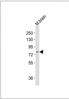
WB (Western Blot) Anti-MeCP2 Antibody (S421) at 1:2000 dilution + mouse brain lysates/proteins at 20 ug per lane. Secondary Goat Anti-Rabbit IgG, (H+L), Peroxidase conjugated at 1/10000 dilution. Predicted band size : 52 kDa. Blocking/Dilution buffer: 5% NFDM/TBST.
