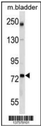
WB (Western Blot) GCLC Antibody (Center) western blot analysis in mouse bladder tissue lysates (35ug/lane).This demonstrates the GCLC antibody detected the GCLC protein (arrow).
