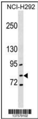
WB (Western Blot) GCLC Antibody (Center) western blot analysis in NCI-H292 cell line lysates (35ug/lane).This demonstrates the GCLC antibody detected the GCLC protein (arrow).
