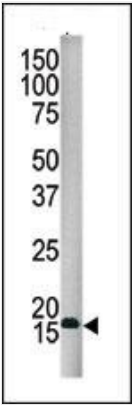
WB (Western Blot) Western blot analysis of SUMO4 Antibody (Center) in HepG2 cell line lysate. SUMO4 (arrow) was detected using the purified Pab.
