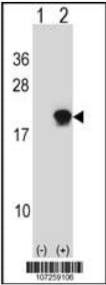
WB (Western Blot) Western blot analysis of SUMO4 (arrow) using rabbit polyclonal SUMO4 Antibody (Center). 293 cell lysates (2 ug/lane) either nontransfected (Lane 1) or transiently transfected (Lane 2) with the SUMO4 gene.
