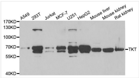
WB (Western Blot) Western blot analysis of extracts of various cell lines, using TKT antibody at 1:1000 dilution. Secondary antibody: HRP Goat Anti-Rabbit IgG (H+L) at 1:10000 dilution. Lysates/proteins: 25ug per lane. Blocking buffer: 3% nonfat dry milk in TBST. Detection: ECL Basic Kit. Exposure time: 60s.
