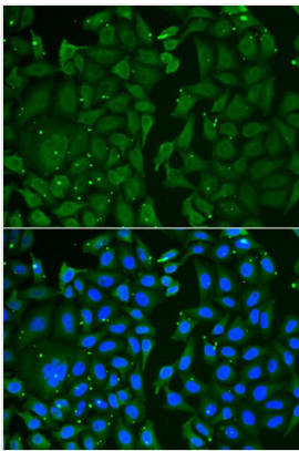
IF (Immunofluorescence) Immunofluorescence analysis of U2OS cells using TKT antibody. Blue: DAPI for nuclear staining.
