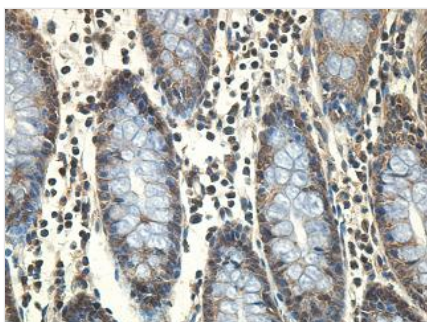
Immunohistochemical staining of formalin-fixed paraffin-embedded fetal colon showing cytoplasmic staining with anti-GRPEL1 antibody at a dilution of 1/100
