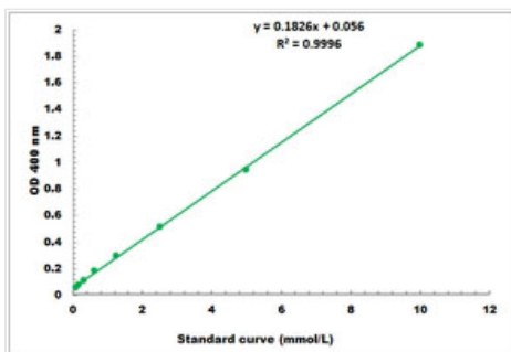
Standard Curve (Sample) Representative Standard Curve
