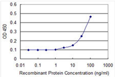
Application Data Detection limit for recombinant GST tagged BANF1 is approximately 10ng/ml as a capture antibody.
