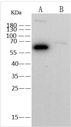
WB (Western Blot) Anti-NP mouse monoclonal antibody at 1 ug/mL. Sample: Recombinant Protein 10 ng Lane A: H3N2 (A/Darwin/9/2021)/(A/Darwin/6/2021) NP Protein Lane B: Influenza B (B/Austria/1359417/2021) NP Protein Secondary Goat Anti-Mouse IgG (H+L)/HRP at 1/10000 dilution Developed using the ECL technique. Performed under reducing conditions.
