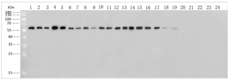
WB (Western Blot) Anti-NP mouse monoclonal antibody at 1:1000 dilution. Sample: Recombinant Protein 10 ng Lane 1: H1N1 (A/Brevig Mission/1/1918) NPLane 2: H1N1 (A/Brisbane/02/2018) NPLane 3: H1N1 (A/California/07/2009) NPLane 4: H1N1 (A/Guangdong-Maonan/SWL1536/2019) NPLane 5: H1N1 (A/Hawaii/70/2019) NPLane 6: H1N1 (A/Michigan/45/2015) NPLane 7: H1N1 (A/Puerto Rico/8/34/Mount Sinai) NP (I116M) Lane 8: H1N1 (A/Victoria/2570/2019)/(A/Wisconsin/588/2019) NPLane 9: H2N2 (A/Ann Arbor/6/1960) NPLane 10: H3N2 (A/Aichi/2/1968) NPLane 11: H3N2 (A/Cambodia/e0826360/2020 (H3N2)-like) NPLane 12: H3N2 (A/Hong Kong/1/1968) NPLane 13: H3N2 (A/Hong Kong/2671/2019) NPLane 14: H3N2 (A/Hong Kong/45/2019) NPLane 15: H3N2 (A/Hong Kong/4801/2014) NPLane 16: H3N2 (A/Kansas/14/2017) NPLane 17: H3N2 (A/Switzerland/9715293/2013) NPLane 18: H7N9 (A/Anhui/1-BALF_RG6/2013) NPLane 19: H7N9 (A/Shanghai/2/2013) NPLane 20: Influenza B (B/Brisbane/60/2008) NPLane 21: Influenza B (B/Colorado/06/2017) NPLane 22: Influenza B (B/Florida/4/2006) NPLane 23: Influenza B (B/Phuket/3073/2013) NPLane 24: Influenza B (B/Washington/02/2019) NP Secondary Goat Anti-Mouse IgG (H+L)/HRP at 1/10000 dilution Developed using the ECL technique. Performed under reducing conditions.
