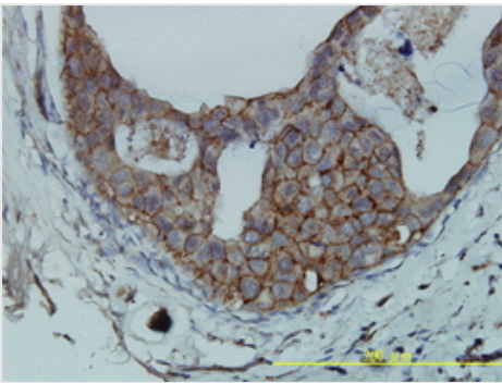
IHC (Immunohistochemistry) Immunoperoxidase of monoclonal antibody to F11R on formalin-fixed paraffin-embedded human breast cancer tissue. [antibody concentration 1ug/ml].
