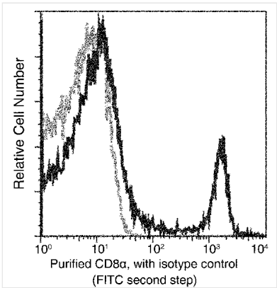
FCM/FACS (Flow Cytometry) Flow cytometric analysis of Mouse CD8alpha expression on BABL/c splenocytes. Cells were stained with purified anti-Mouse CD8alpha, then a FITC-conjugated second step antibody. The fluorescence histograms were derived from gated events with the forward and side light-scatter characteristics of intact cells.
