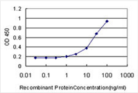
Application Data Detection limit for recombinant GST tagged SPP1 is ~1ng/ml as a capture antibody.
