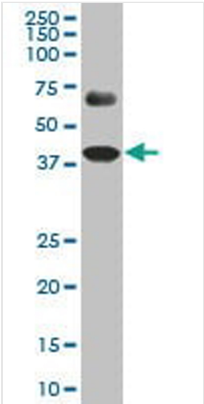
WB (Western Blot) SPP1 monoclonal antibody. Western Blot analysis of SPP1 expression in human stomach.
