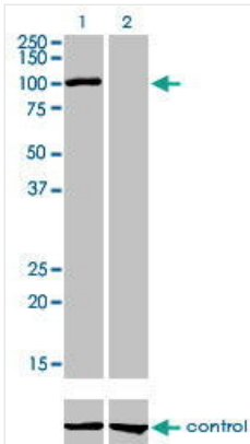
WB (Western Blot) Western Blot analysis of AHR over-expressed 293 cell line, cotransfected with AHR Validated Chimera RNAi (Lane 2) or non-transfected control (Lane 1). Blot probed with 123091. GAPDH (36.1kD) used as specificity and loading control.
