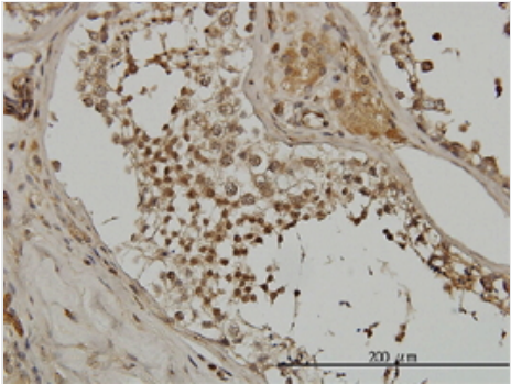
IHC (Immunohistochemistry) Immunoperoxidase of monoclonal antibody to ACTN4 on formalin-fixed paraffin-embedded human testis. [antibody concentration 3ug/ml].
