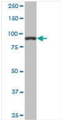
WB (Western Blot) ACTN4 monoclonal antibody Western Blot analysis of ACTN4 expression in NIH/3T3.
