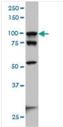
WB (Western Blot) ACTN4 monoclonal antibody Western Blot analysis of ACTN4 expression in HeLa NE.
