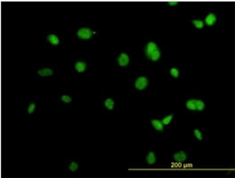
IF (Immunofluorescence) Immunofluorescence of monoclonal antibody to ACTN4 on HeLa cell. [antibody concentration 20ug/ml].
