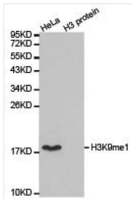
WB (Western Blot) Western blot analysis of extracts of HeLa cell line and H3 protein expressed in E.coli., using H3K9me1 antibody.
