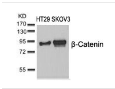
WB (Western Blot) Western blot analysis of extracts from HT29 and SKOV3 cells using b-Catenin(Ab-37) Antibody.
