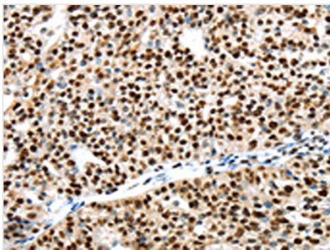
IHC (Immunohistochemistry) The image on the left is immunohistochemistry of paraffin-embedded Human breast cancer tissue using AAA241905(UBA1 Antibody) at dilution 1/40, on the right is treated with synthetic peptide. (Original magnification: ×200)
