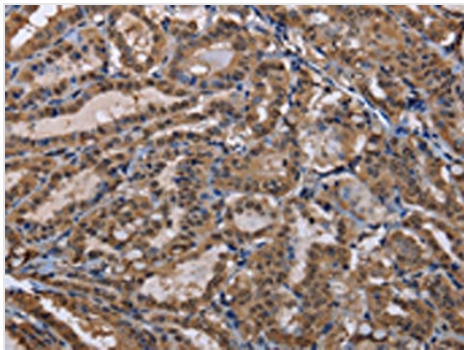
IHC (Immunohistochemistry) The image on the left is immunohistochemistry of paraffin-embedded Human thyroid cancer tissue using AAA237330(CUL3 Antibody) at dilution 1/30, on the right is treated with fusion protein. (Original magnification: ×200)
