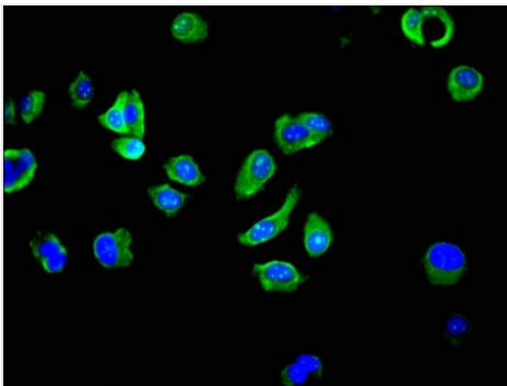
IF (Immunofluorescence) Immunofluorescent analysis of MCF-7 cells using AAA233704 at a dilution of 1:100 and Alexa Fluor 488-conjugated AffiniPure Goat Anti-Rabbit IgG(H+L)
