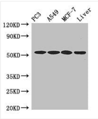
WB (Western Blot) Western BlotPositive WB detected in: PC3 whole cell lysate,A549 whole cell lysate,MCF-7 whole cell lysate,,Mouse liver tissueAll lanes: IRF6 antibody at 4ug/mlSecondaryGoat polyclonal to rabbit IgG at 1/50000 dilutionPredicted band size: 54,42 KDaObserved band size: 54 KDa
