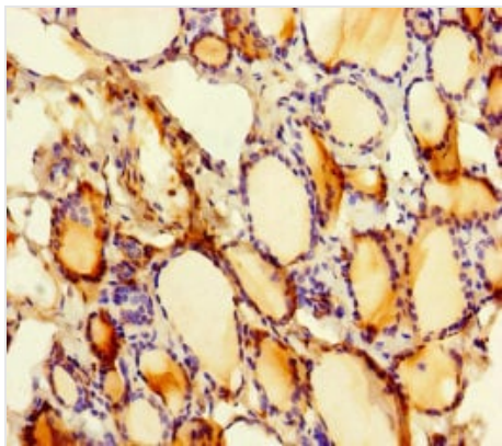
IHC (Immunohistochemistry) Immunohistochemistry of paraffin-embedded human thyroid tissue using AAA229307 at dilution of 1:100
