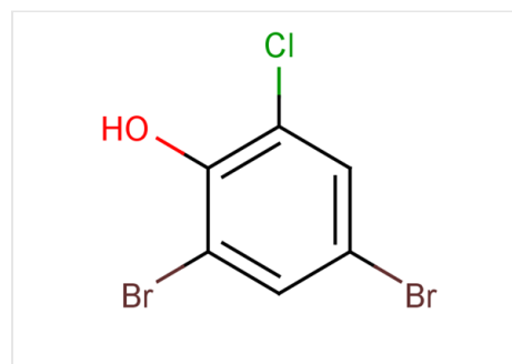
Structure 6-Chloro-2,4-dibromophenol, CAS 4526-56-1
