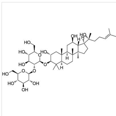
Structure Gyenoside LI, CAS 94987-10-7
