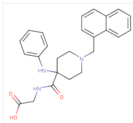
Structure VBIT-12, CAS 2089227-65-4
