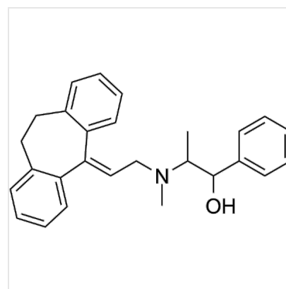
Structure Trecadrine, CAS 90845-56-0
