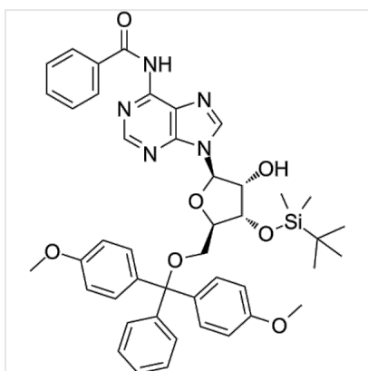
Structure 5'-DMT-3'-TBDMS-Bz-rA, CAS 81256-88-4
